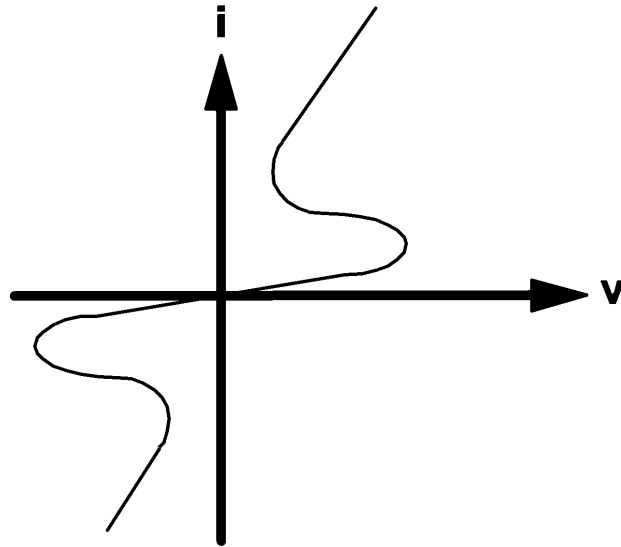
4.2 Example of a type of v - i characteristics that can be described as a current-defined resistor.
