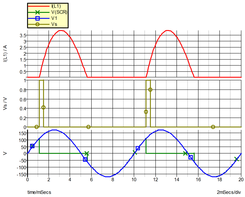
9.23 Waveforms for Example 7
